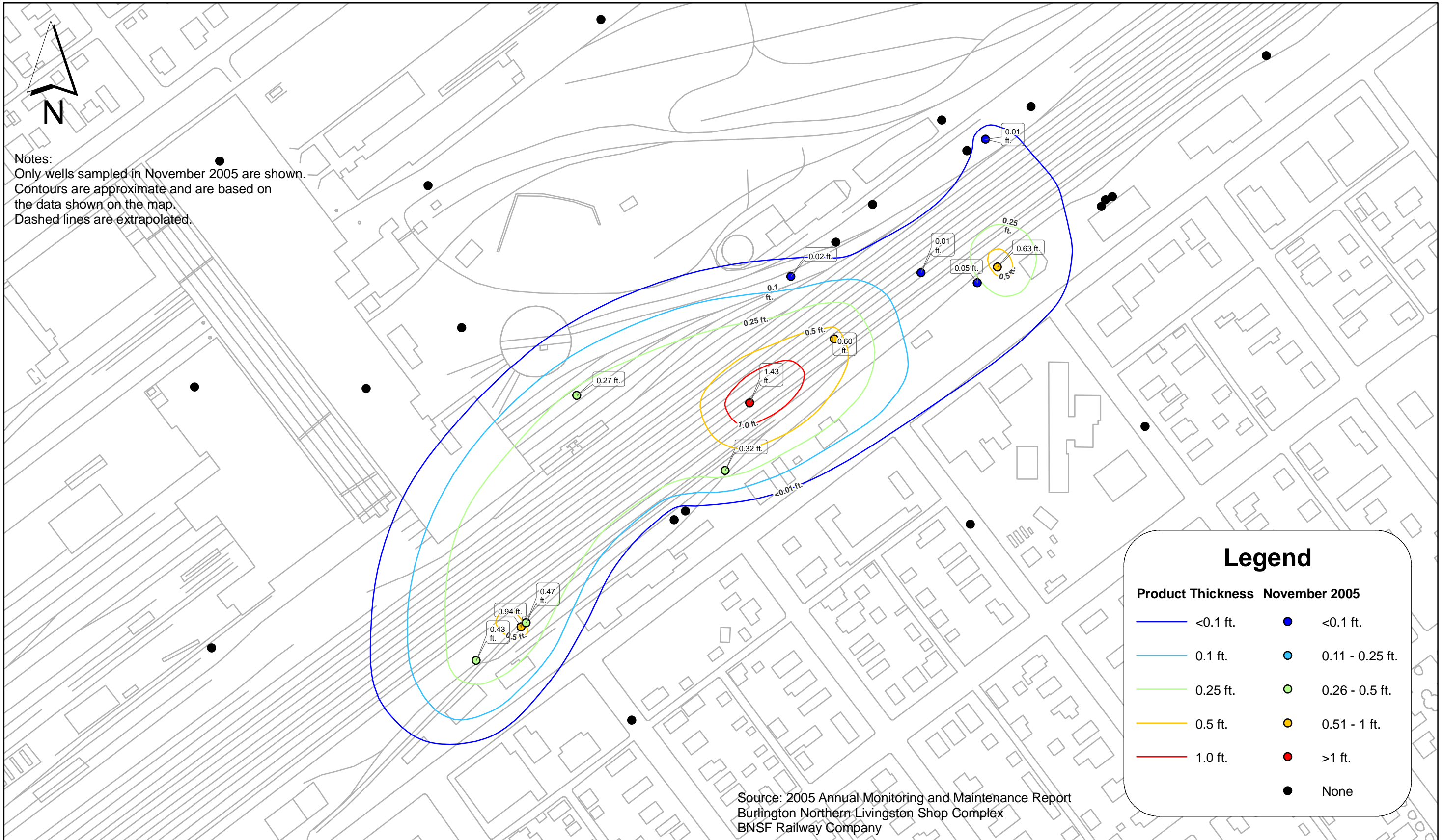
Floating Product in Ground Water - November 2005 BN Livingston Shop Complex Livingston, Montana
